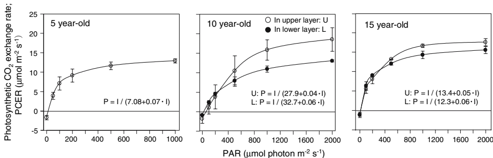
Fig. 1 Light response of photosynthetic CO 2 exchange rate (PCER) measured at leaf temperature of 30°C in the leaves of Kandelia candel in 5-, 10-, and 15-year-old stand. In the leaves
