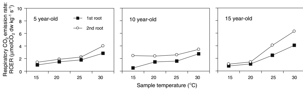
Fig. 5 Temperature response of respiratory CO 2 emission rate (RCER) of roots in three kinds of stand age. The values of RCER here were calculated in the unit of dry weight of roots
