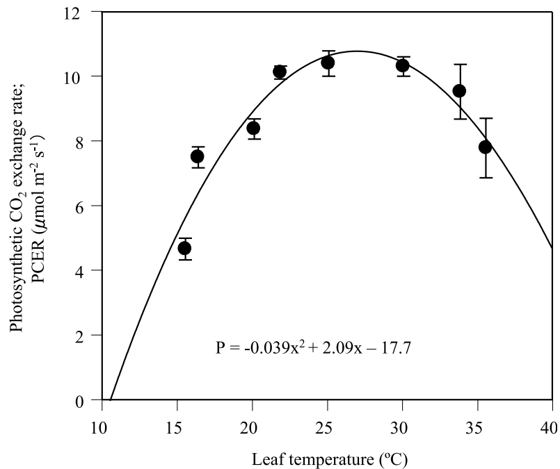
Fig. 2. Influence of temperature on photosynthetic CO 2 exchange rate (PCER) measured in the leaves of Rhizophora stylosa in Ishigaki, Japan. A quadratic curve in the graph was a regression curve. Vertical bars are standard deviations.
