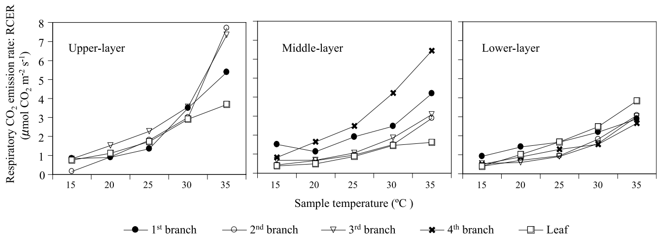
Fig. 5. Influence of temperature on respiratory \text{CO}_2 emission rate (RCER) of each organ in three layers of Rhizophora stylosa canopy in Ishigaki, Japan. The values of RCER in the graph were calculated per unit surface area of each organ. The branch was divided into four offshoot groups; first, second, third, and fourth offshoots.
