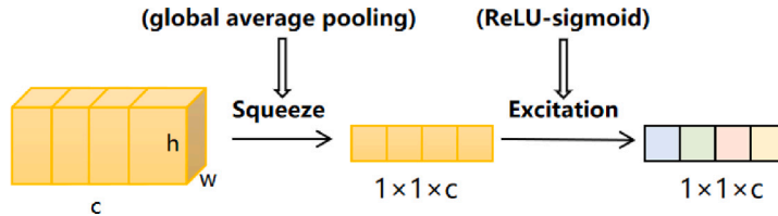
Fig. 9. Structure of SEWeight module which includes the two most important components: Squeeze and Excitation.
