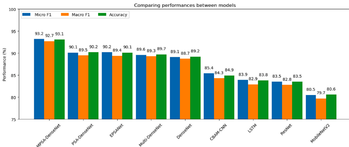
Fig. 13. Micro F_1 , Macro F_1 , and accuracy of nine models on test set.
