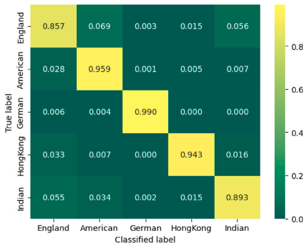
Fig. 12. Normalized confusion matrix for accent classification by MPSA-DenseNet on test set.
