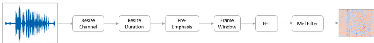
Fig. 3. Voice file standardization and spectrogram conversion with MFCCs.
