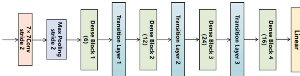
Fig. 5. DenseNet-121 architecture.
